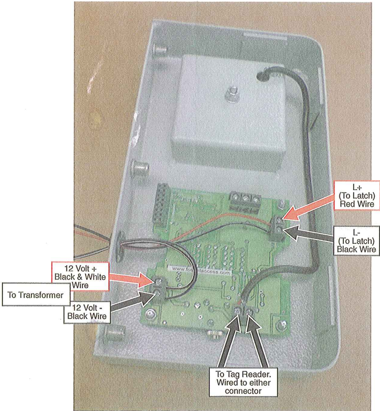
Back view of Reader Box with back panel removed for connecting wiring
